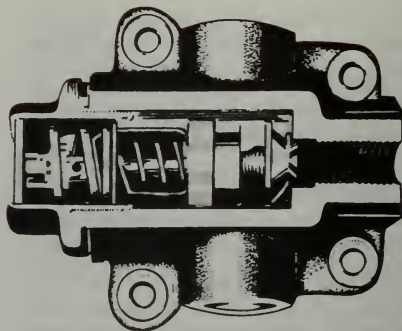
FIGURE 6-28. A typical thermostatic bypass valve.
